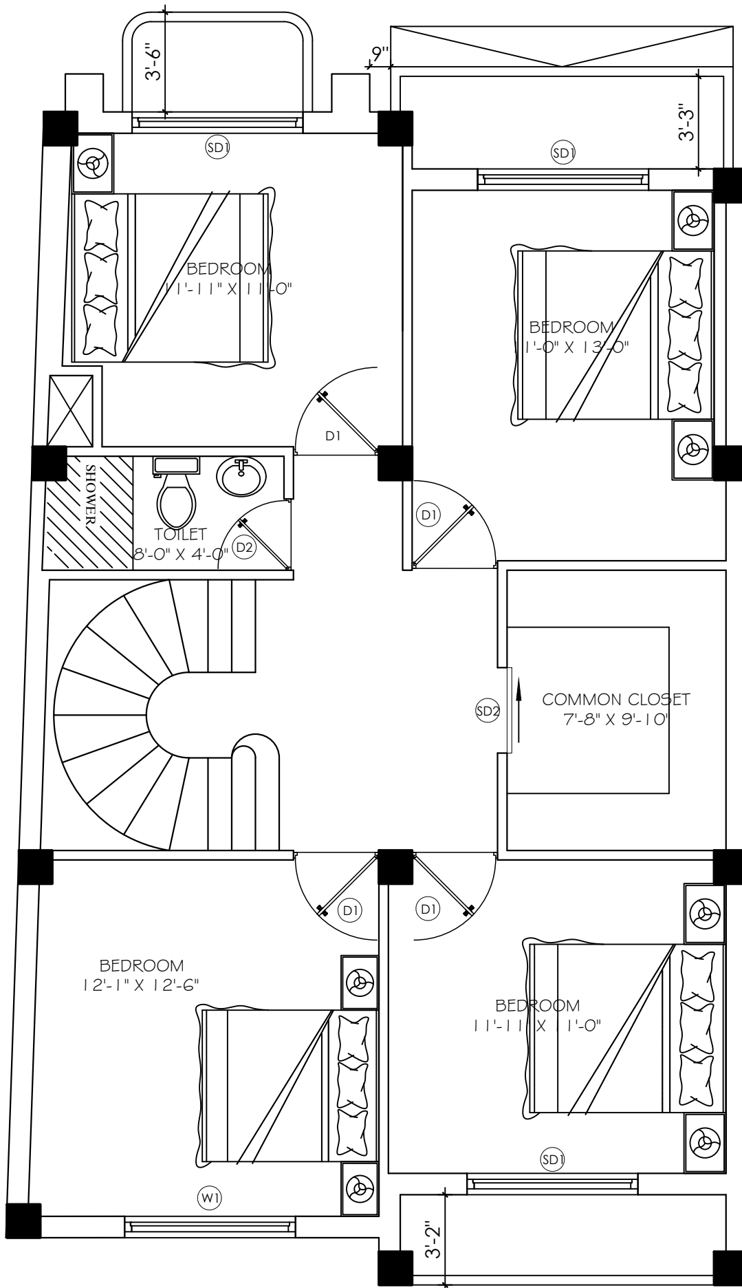
SECOND FLOOR PLAN FAR COUNTABLE AREA: 964.76 SQ.FT FAR NON COUNTABLE AREA : 99.73 SQ.FT TOTAL AREA : 1064.49 SQ.FT
